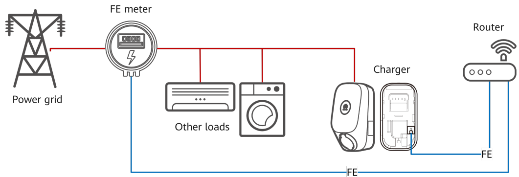
Figure 5-2 Charger FE port directly connected to a router
